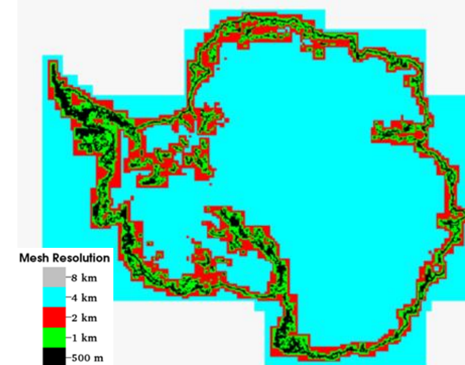
AMR benefits: Only ~1% of domain is covered with 500m mesh (in black). In many scenarios, refined meshes sweep over much of the WAIS as they follow retreating grounding lines.
