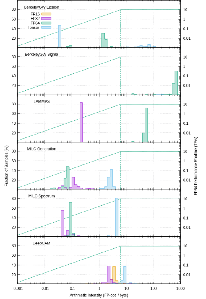
Fig. 2. Algorithmic Intensity distributions for the NERSC-10 GPU benchmarks.
