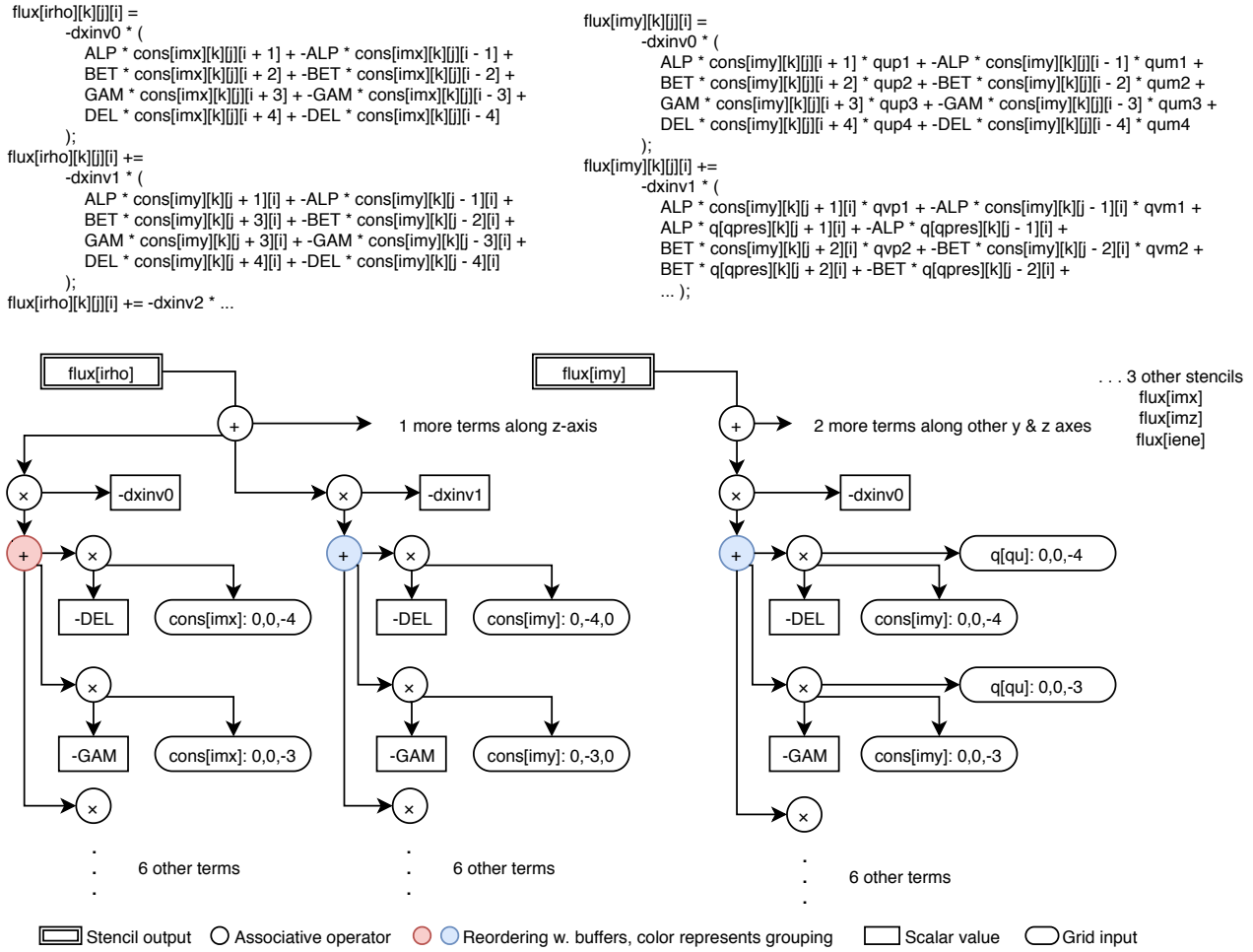
Figure 1: CNS's hyperterm stencil excerpt (top) and derived expression trees (bottom).
