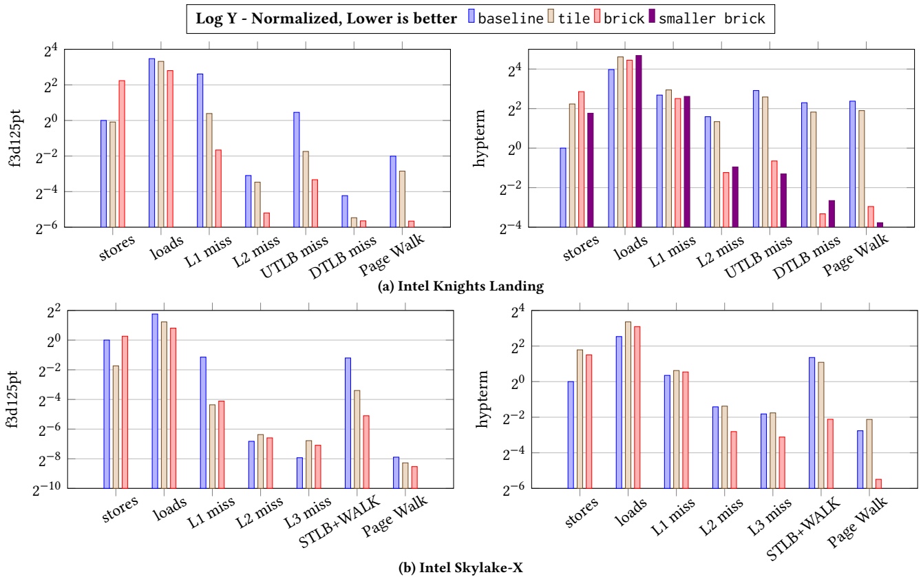
Figure 8: Profiling metrics on KNL and Skylake-X. Each bar is the raw counter value, normalized to the baseline total number of stores. The generated code provides a dramatic reduction in cache and TLB misses and page walks. On KNL, L1 L2 and TLB misses are reduced as much as 19×, 7×, and 49× respectively. On Skylake-X, we also reduced L1 misses by up to 8× and TLB-related metrics up to 14×. These indicates much better data locality and cache reuse.
