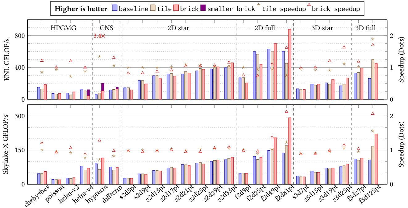
Figure 7: Performance on KNL and Skylake-X. For real-world stencil kernels, smaller blocking sizes may be beneficial because more input grids can put higher pressure on the cache. For higher-order and real-world stencils, the brick approach often provides the best speedup: On KNL, hypterm – 3.4× and f3d125pt – 1.9×. On Skylake-X, hypterm – 1.3× and f3d125pt – 2.1×.
