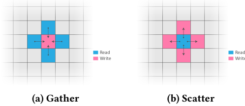
Figure 3: Gather vs. scatter operations for 5 points in 2D.
