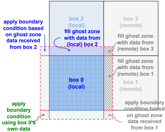
Figure 2. 2D illustration of the ghost zone exchange and boundary condition in the 3D HPGMG-FV.
