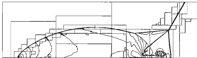
FIG. 8. Density contours from a higher order Godunov/AMR computation for the flow displayed in Fig. 7.
