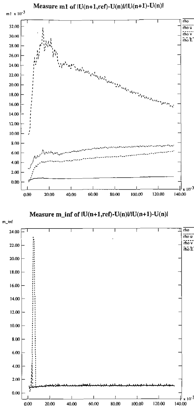
FIG. 13. Values of m_1 (top) and m_\infty (bottom) from a computation of a Mach 10 flow past a 30^\circ ramp on a 240 \times 200 uniform grid in which the ramp is represented as an inclined Cartesian fluid/body interface as in Fig. 7.
