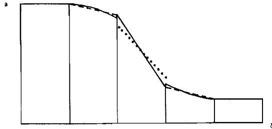
FIG. 3. PPM discontinuity detection. The central zone in this figure is judged to be within a discontinuity, according to the detection criterion given in Eqs. (1.15)–(1.17) of the text. The usual interpolated zone structure shown by the dotted line is therefore replaced by the steeper structure shown by the solid line. The two edge values joined by this line are obtained from the linear distributions in the neighboring zones, which are indicated by the dashed lines. A monotonicity constraint on these linear distributions has kept their slopes small and caused the distribution derived for the central zone to be quite steep.
