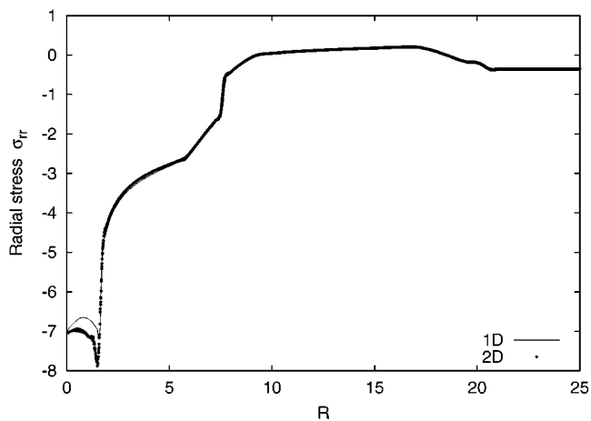
FIG. 13. \sigma_{rr} at time 4.
