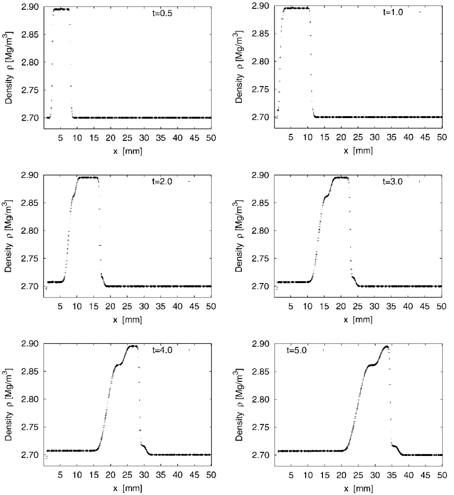
FIG. 8. Mass density \rho for Wilkins's problem with impact velocity 0.8 km/s. Time in \mu s.
