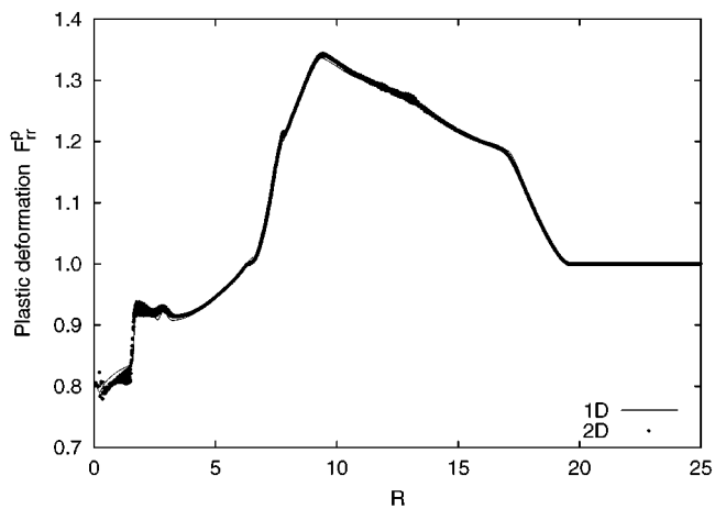
FIG. 14. \mathcal{F}^p_{rr} component of plastic deformation tensor.
