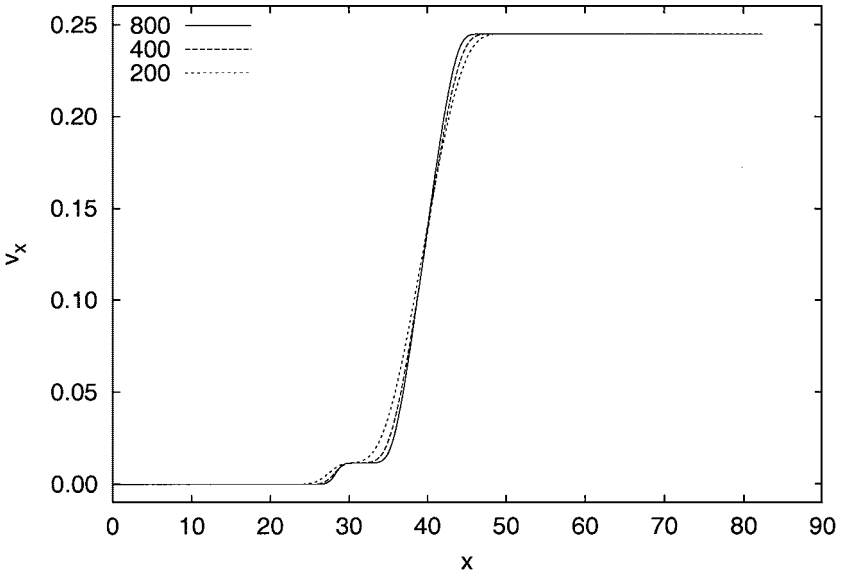
FIG. 14. Velocity for one-dimensional solid–vacuum Riemann problem.
