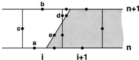
FIG. 19. Centroid-centered second-order fluxes give a first-order-accurate ( \mathcal{O}(h) ) difference scheme.
