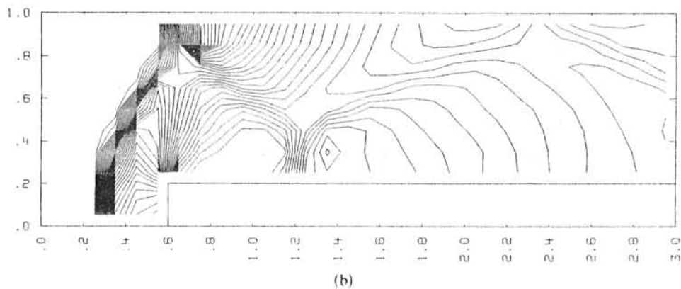
FIG. 4. Contour plots for two-dimensional test problem, \Delta x = .1 . a) Density, 30 contours between .98 and 6.38. b) Pressure, 30 contours between 1.11 and 11.6.
