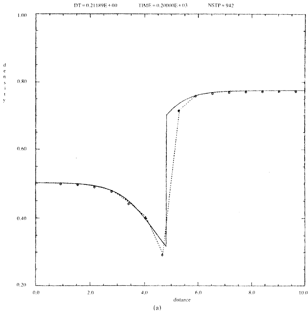
FIG. 3. Steady state density profiles for one-dimensional duct problem. a) \Delta r = \frac{5}{8} , b) \Delta r = \frac{5}{16} .
