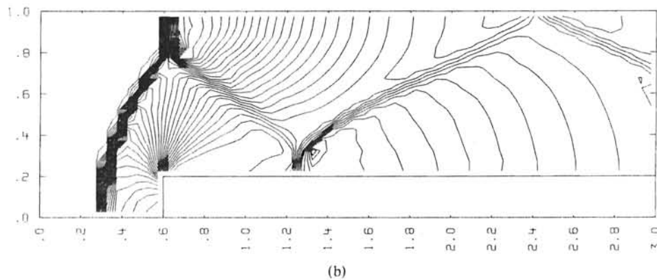
FIG. 5. Contour plots for two-dimensional test problem, \Delta x = .05 . a) Density, 30 contours between .68 and 6.29. b) Pressure, 30 contours between .72 and 11.8.
