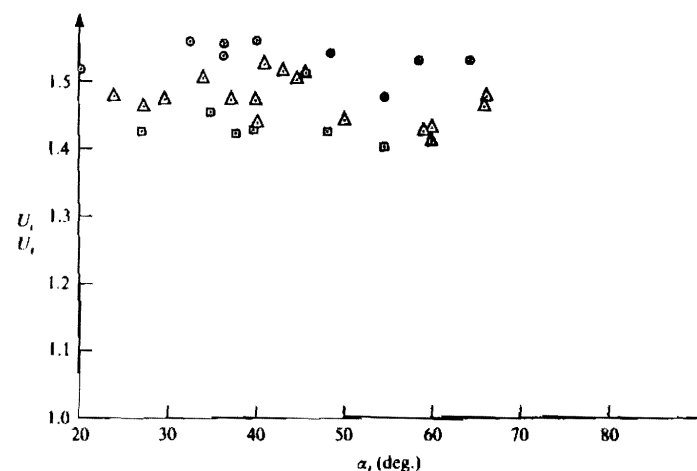
FIGURE 7. Comparison of the wave speed ratio U_t'/U_t (see figure 2c) for a \text{CO}_2/\text{CH}_4 gas interface with \xi_i = 0.78 . \circ , Computed data for pure gases; \square , computed data for 10% contamination of the \text{CH}_4 by the \text{CO}_2 ; \Delta , experimental data (from Abd-El-Fattah & Henderson 1978b).
