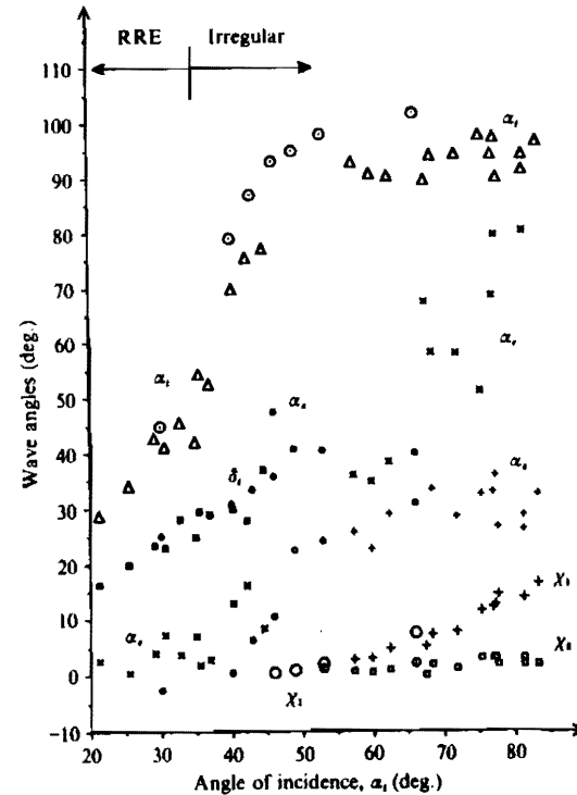
FIGURE 12. Experimental and computational wave angle data for a \text{CO}_2/\text{CH}_4 refraction with \xi_i = 0.18 . Circular symbols represent data from computations with pure gases. All other symbols represent experimental data. \circ, \triangle , Transmitted shock angle \alpha_1 ; \circ, \times , reflected wave angle \alpha_2 , or \alpha_2' ; \bullet, + , side shock angle \alpha_3 ; \circ, \square , interface deflection angle \delta_1 ; \circ, + , trajectory path angle \chi_1 ; \circ, \square , trajectory path angle \chi_2 . (Experimental data from Abd-El-Fattah & Henderson 1978b.)
