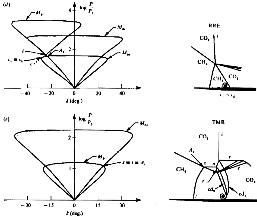
FIGURE 10. Polar diagrams for a strong shock refraction sequence with \xi_i = 0.18 at a pure \text{CO}_2/\text{CH}_4 gas interface. (a) RRE, \epsilon_1 solution at \alpha_1 = 30^\circ ; (b) RRE, \epsilon_1 solution at \alpha_1 = \alpha_{nc} = 35.95^\circ . Note that \epsilon_1 is not a continuation of either the \lambda_1 , or \lambda_2 solutions, therefore the shock critical angle for \lambda_1 \equiv \lambda_2 is irrelevant for transition to irregular refraction in this case; (c) RRE, at \alpha_1 = 37^\circ ; note there are now two RRE solutions, \epsilon_1 and \epsilon_2 ; the \epsilon_1 solution is observed in experiments; (d) RRE, at the relevant shock critical angle, \epsilon_1 \equiv \epsilon_2 , \alpha_1 = \alpha_{nc} = 46.204^\circ ; this is the transition condition for RRE \rightleftharpoons TMR; (e) twin Mach reflection-refraction TMR at \alpha_1 = 60^\circ > \alpha_{nc} .
