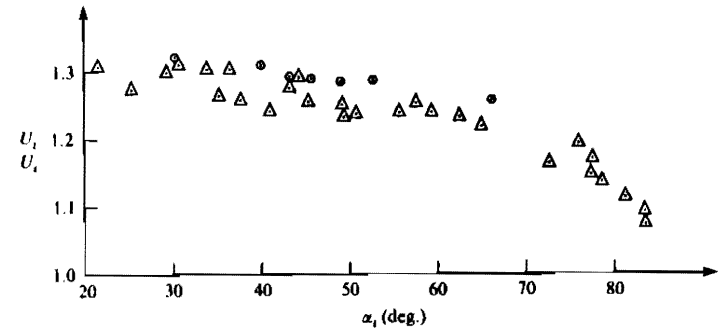
FIGURE 11. Comparison of the wave speed ratio U_2/U_1 (see figure 2c) for a \text{CO}_2/\text{CH}_4 gas interface with \xi_i = 0.18 . \circ , Computed data for pure gases; \triangle , experimental data (from Abd-El-Fattah & Henderson 1978b).
