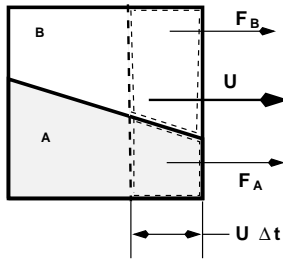
FIG. 1. Illustration of advection of interface. The volume fluxed out of the cell during a time step \Delta t is shown by the dashed rectangle. The quadrilateral volume of fluid 1 and fluid 2 with this rectangle are the volume fluxes ( F_{V\alpha} ) of fluid 1 and fluid 2 during the time step.
