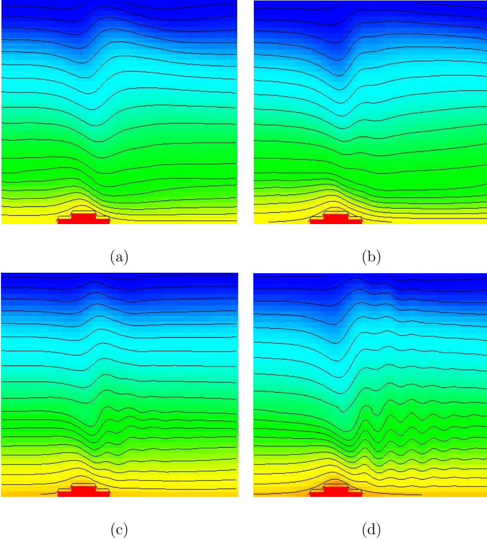
Figure 5: Isentropes for a two-layered atmosphere flowing over a 600\text{ m} high mountain at t = 10000\text{ s} for an interface at a quarter wavelength (a) \Delta t = 30\text{ s} with filtering and (b) \Delta t = 15\text{ s} with no filtering, and for an interface at a half wavelength (c) \Delta t = 30\text{ s} with filtering and (d) \Delta t = 15\text{ s} with no filtering.
