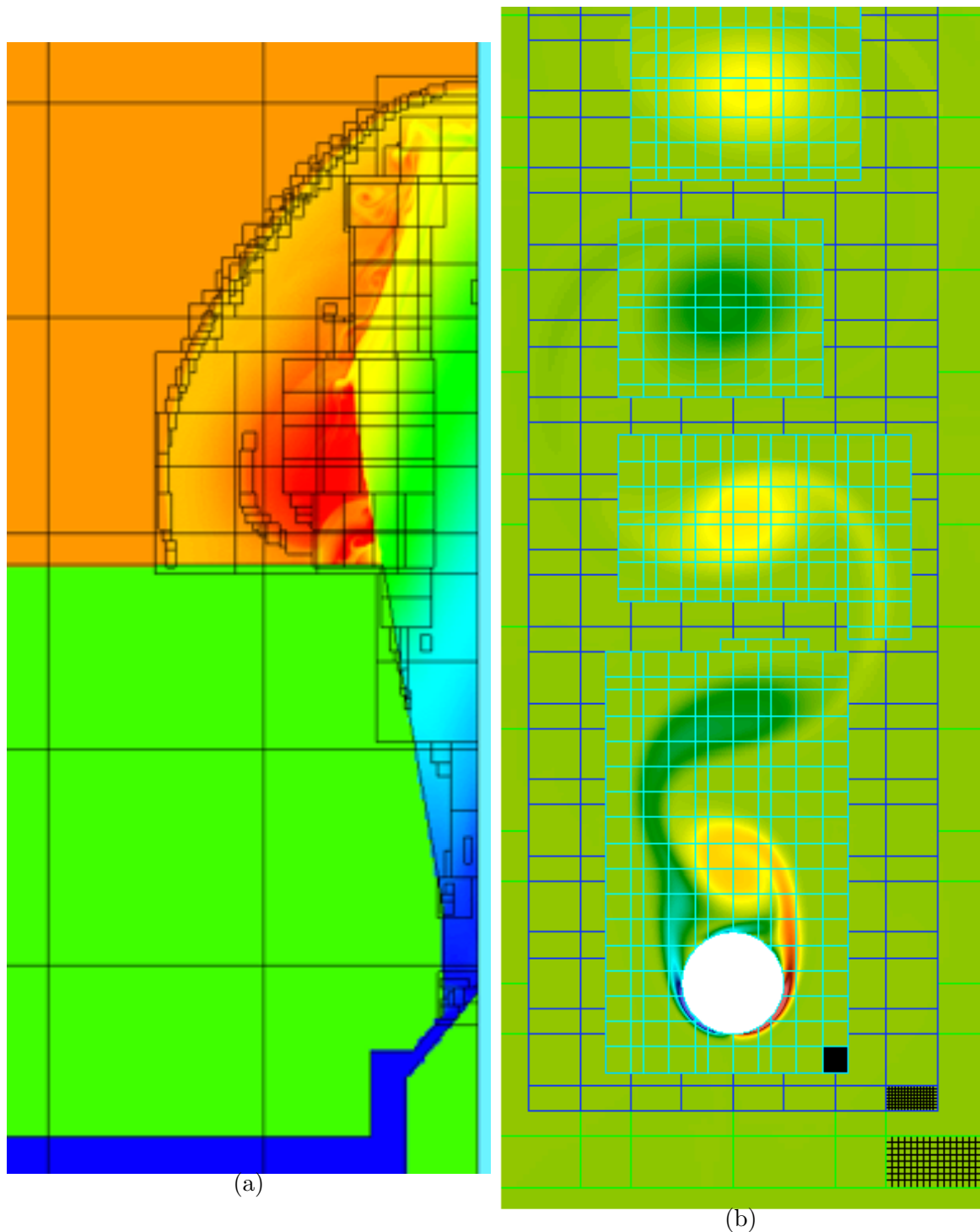
Figure 4. (a) Compressible gas dynamics flow from high pressure reservoir into a vacuum through a nozzle. (b) Kármán vortex street behind cylinder at Re=300 . Effective fine grid resolution 2048x4096. Color scaled for magnitude of vorticity [-175, 175] . Images made with the VisIt visualization package.
