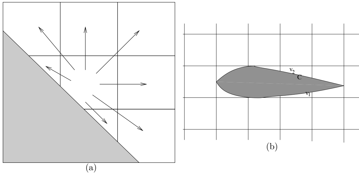
Figure 3. (a) Redistribution of nonconservative update to neighboring cells (b) Coarsened EBIndexSpace showing a multivalued cell
