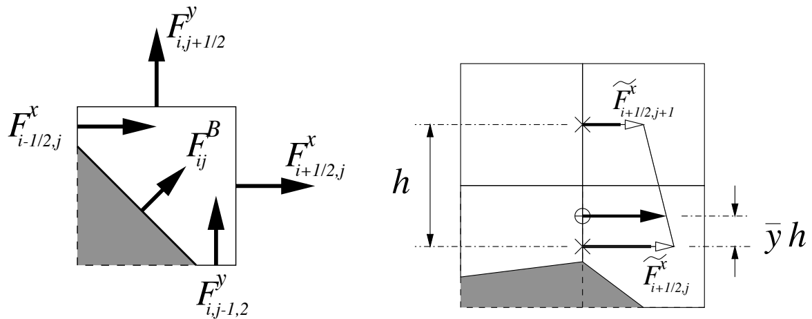
Figure 1. Left: fluxes that make up a conservative update of an irregular cell. Right: constructing a non-unit area fraction aperture flux by interpolation.
