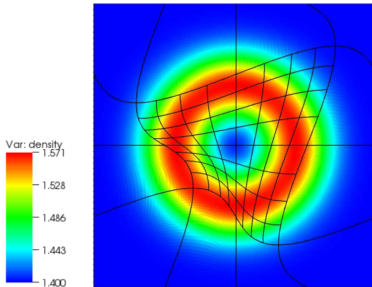
Figure 2. Plot of density with a Gaussian acoustic pulse in a polytropic gas in a periodic domain, using two levels of refinement with the mapped coordinates of (21), after 240 coarse-level time steps each of length 0.0006. At the initial time, the density profile is a circularly symmetric Gaussian with its peak at the center of the domain. Each grid box consists of 32 \times 32 cells; the outlines of these boxes are shown in black.
