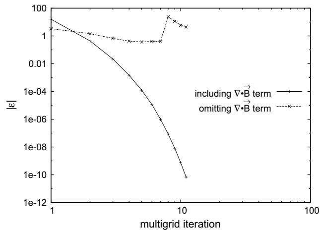
Fig. 9. Multigrid convergence in three dimensions with and without \nabla \cdot \vec{B} term in the flux. \frac{1}{\sigma} = 1 .
