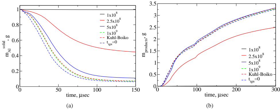
Figure 2: Mass of (a) solid Al, (b) Al products remaining with time.
