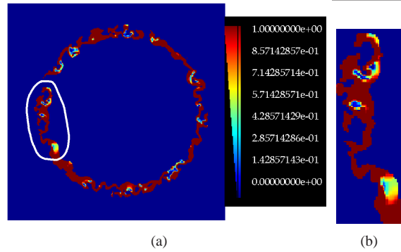
Figure 3: Color scale visualization of the cross-section of the ignition variable f at 18 \mu\text{sec} for the case with A = 1 \cdot 10^9 . The white circled region from (a) is magnified and presented in (b), showing the corrugated ignition front.
