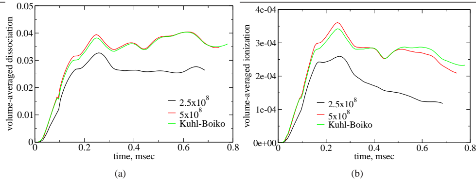
Figure 6: Volume averaged degrees of dissociation and ionization.
