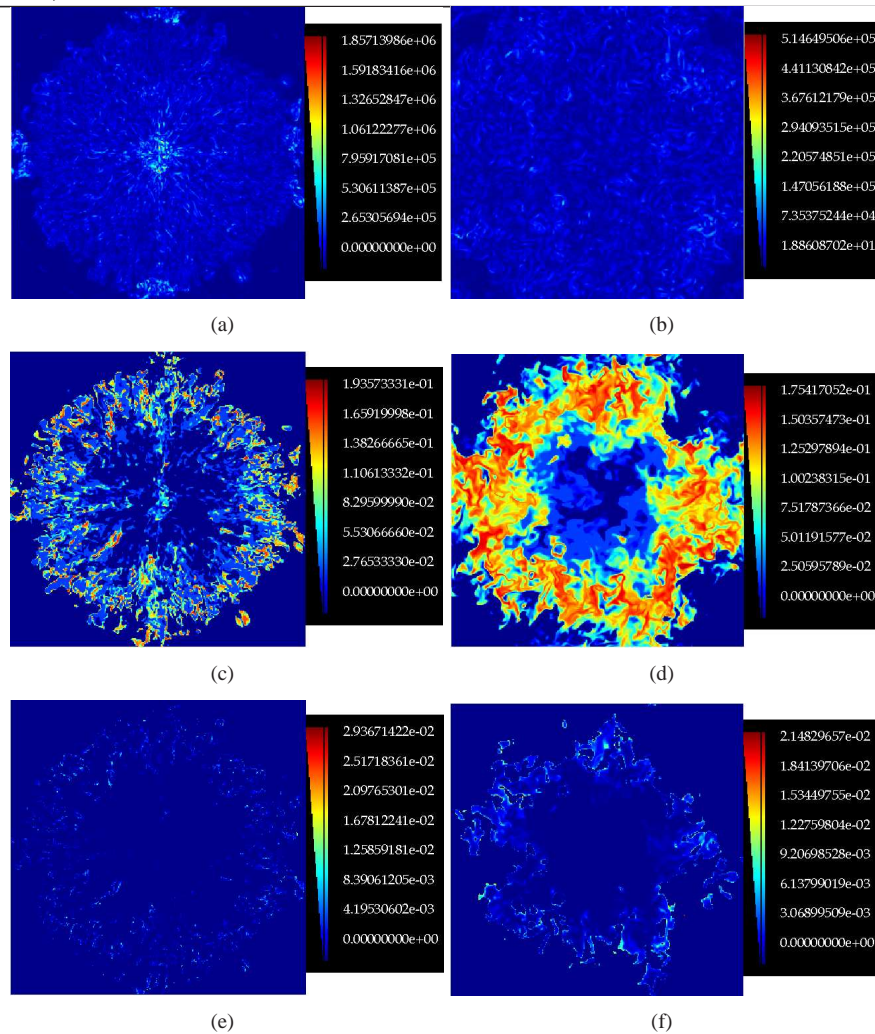
Figure 5: Vorticity (a & b), degree of dissociation (c & d) and degree of ionization (e & f) with the Kuhl-Boiko curve-fit: (a), (c) & (e) at 0.096 msec; (b), (d) & (f) at 0.778 msec.
