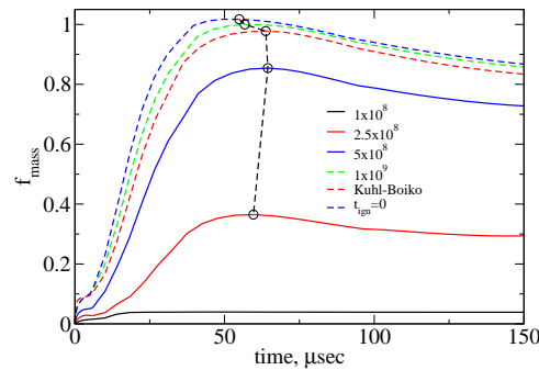
Figure 4: Mass-averaged ignition variable f_{mass} for the different cases considered. The legend denotes the values of A for temperatures higher than 2000 K. The black dashed line joins the peaks.
