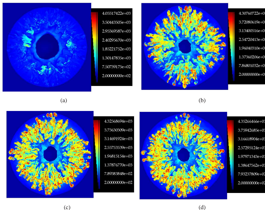
Figure 1: Color scale visualization of a cross-section of the gas temperature field at 70 \mu\text{sec} for different assumed values of A : (a) 1 \cdot 10^8 ; (b) 2.5 \cdot 10^8 ; (c) 1 \cdot 10^9 ; (d) Kuhl-Boiko. The scale denotes the gas temperature in K.
