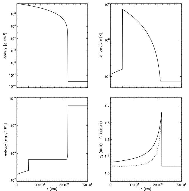
FIG. 1.— White dwarf atmosphere initial model. Shown are the density ( top left ), temperature ( top right ), entropy ( bottom left ), and adiabatic indices ( bottom right ). To prevent convective motions from hitting the lower boundary in our multidimensional tests, the first 5 \times 10^7 \text{ cm} of this model is constructed to have a convectively stable entropy profile. The one-dimensional tests do not use this portion of the model.
