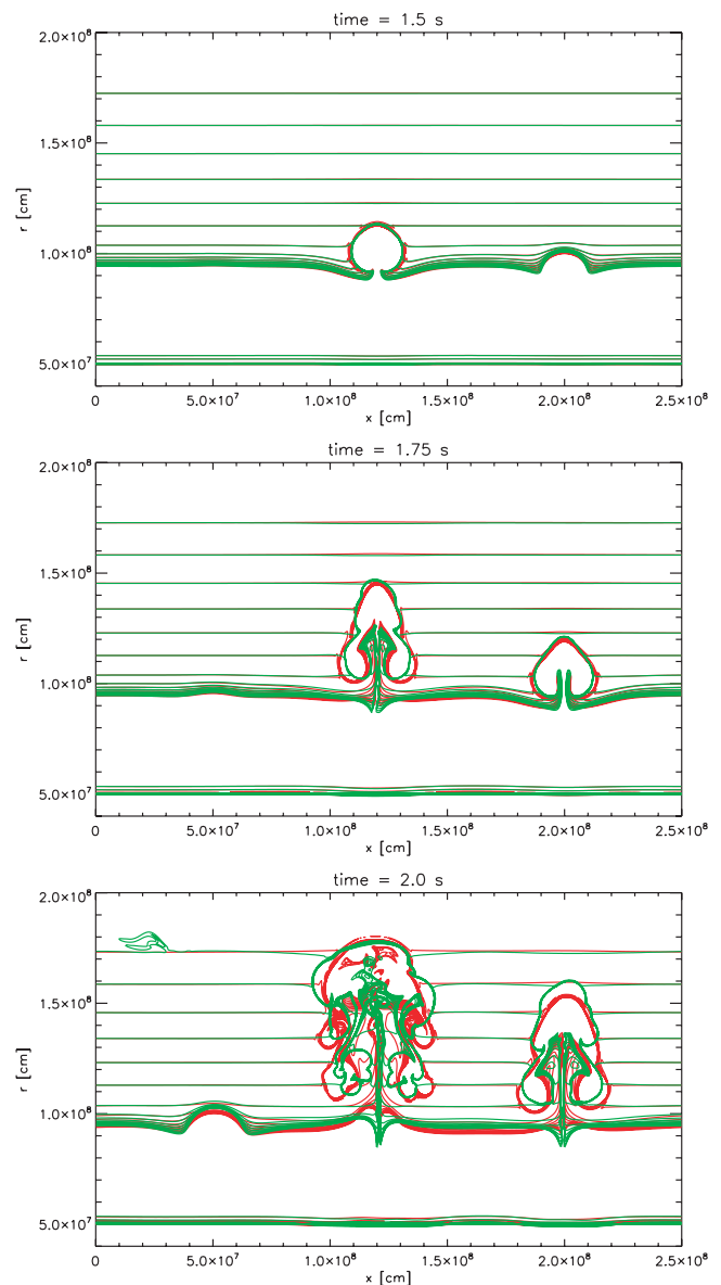
FIG. 6.—Third test case: temperature contours for the low Mach number (green) and unsplit (red) solvers. Here, in addition to the localized heating from the previous test (see Fig. 4), there is a uniform heating layer centered at a height of 7.5 \times 10^7 cm, as specified by eq. (26). Contours span 10^8 to 8 \times 10^8 K, spaced every 5 \times 10^7 K.
