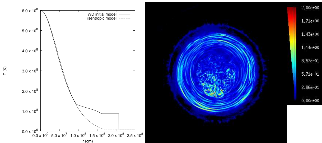
Figure 2. Temperature of the initial model compared to an isentropic model (left) and vorticity (X-Z slice) after 814 s of evolution (right) for the convecting WD problem. (Note that the scale for the vorticity has been reduced from the peak value of 3.27 to enhance detail.)
