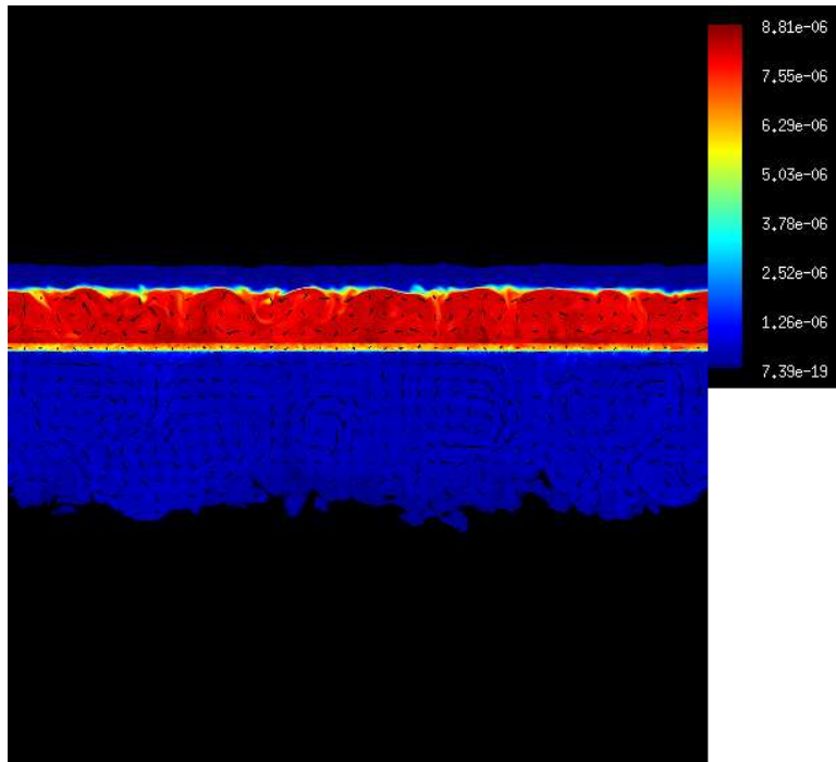
Figure 1. Carbon mass fraction over-plotted with velocity vectors after 0.022 s of evolution for the XRB convection problem. (Note we have zoomed in on the convective region—the total vertical extent of the image is 850 cm.)
