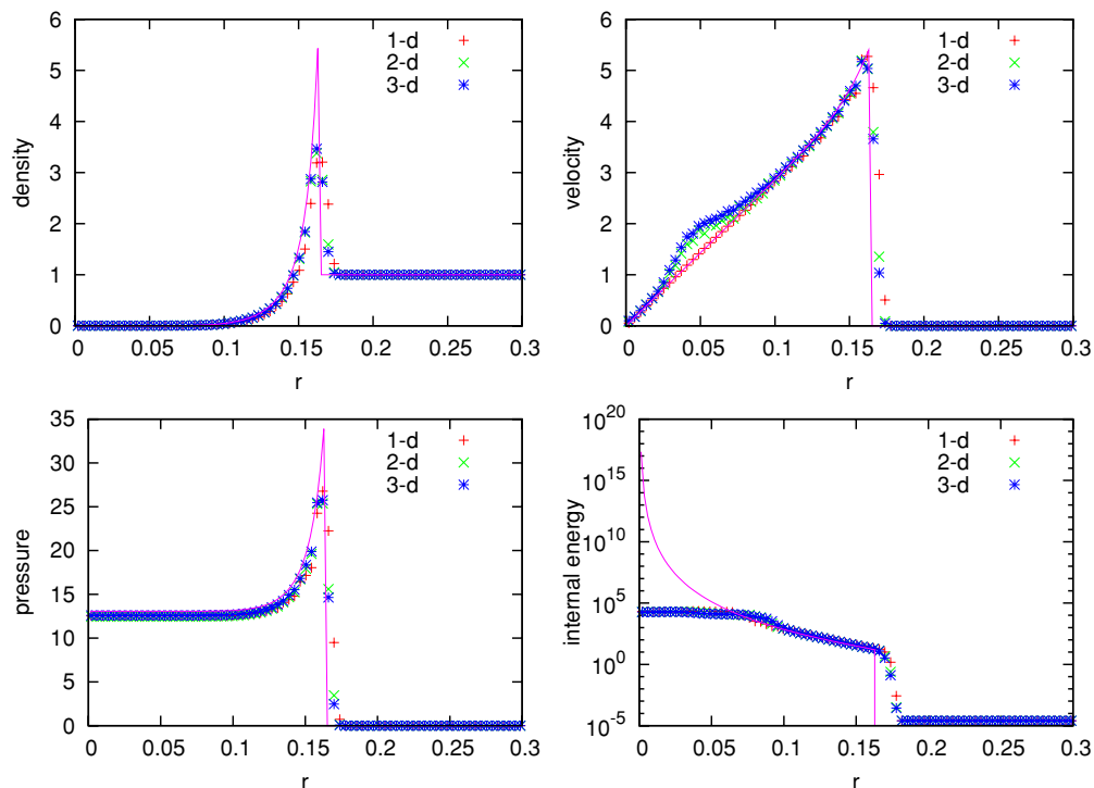
Figure 6. CASTRO solution at t = 0.01 s for the spherical Sedov blast wave problem run in one-dimensional spherical, two-dimensional axisymmetric, and three-dimensional Cartesian coordinates. This was run with a base grid with \Delta x = 0.03125 cm and three levels of factor 2 refinement for an effective resolution of \Delta x = 0.00390625 cm.
