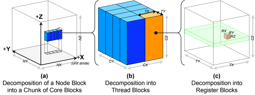
Fig. 3. Four-level problem decomposition: In (a), a node block (the full grid) is broken into smaller chunks . One core block from the chunk in (a) is magnified in (b). A single thread block from the core block in (b) is then magnified in (c) and decomposed into register blocks.
