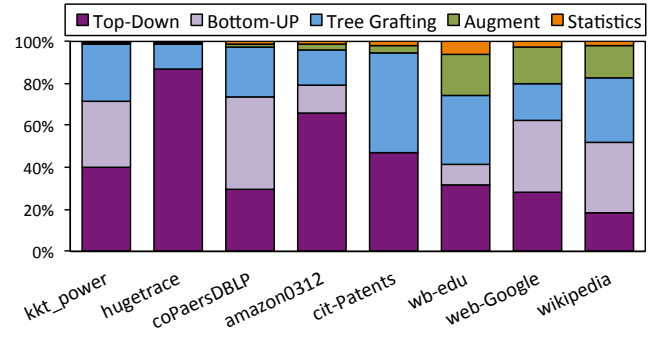
Fig. 6. Breakdown of time spent on different steps of the MS-BFS-Graft algorithm for different graphs on Mirasol with 40 threads.
