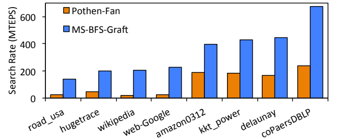
Fig. 4. Search rates of the MS-BFS-Graft and Pothen-Fan algorithms for different input graphs on Mirasol with 40 threads.
