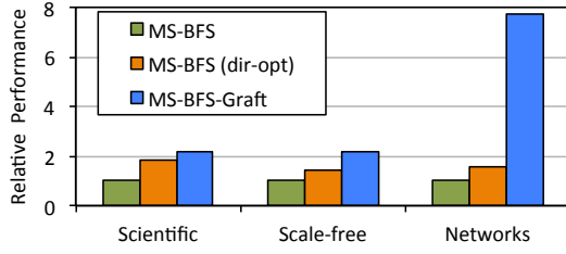
Fig. 7. Performance improvement of the parallel MS-BFS algorithm by direction-optimized BFS and tree-grafting for different classes of graphs on Mirasol with 40 threads.
